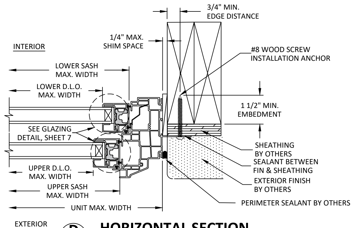
D 4 HORIZONTAL SECTION NAIL FIN INSTALLATION WOOD BUCK
