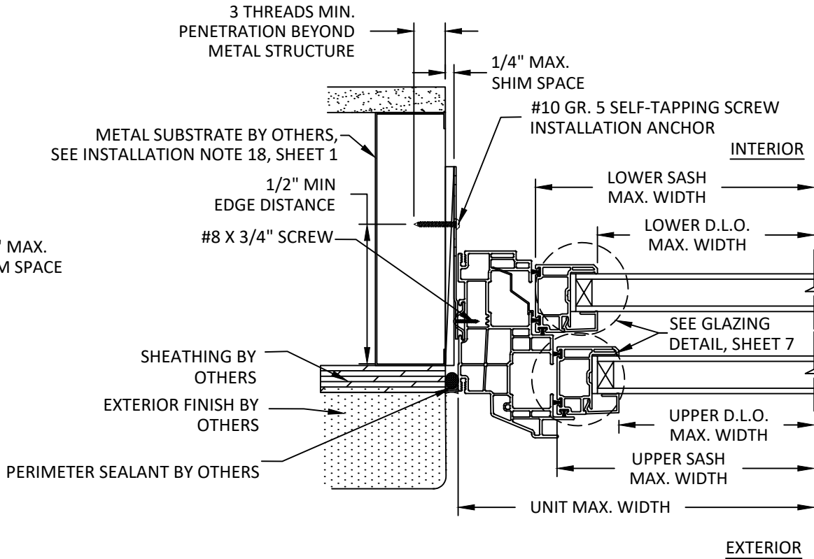
B 6 HORIZONTAL SECTION CLIP INSTALLATION METAL STUD
