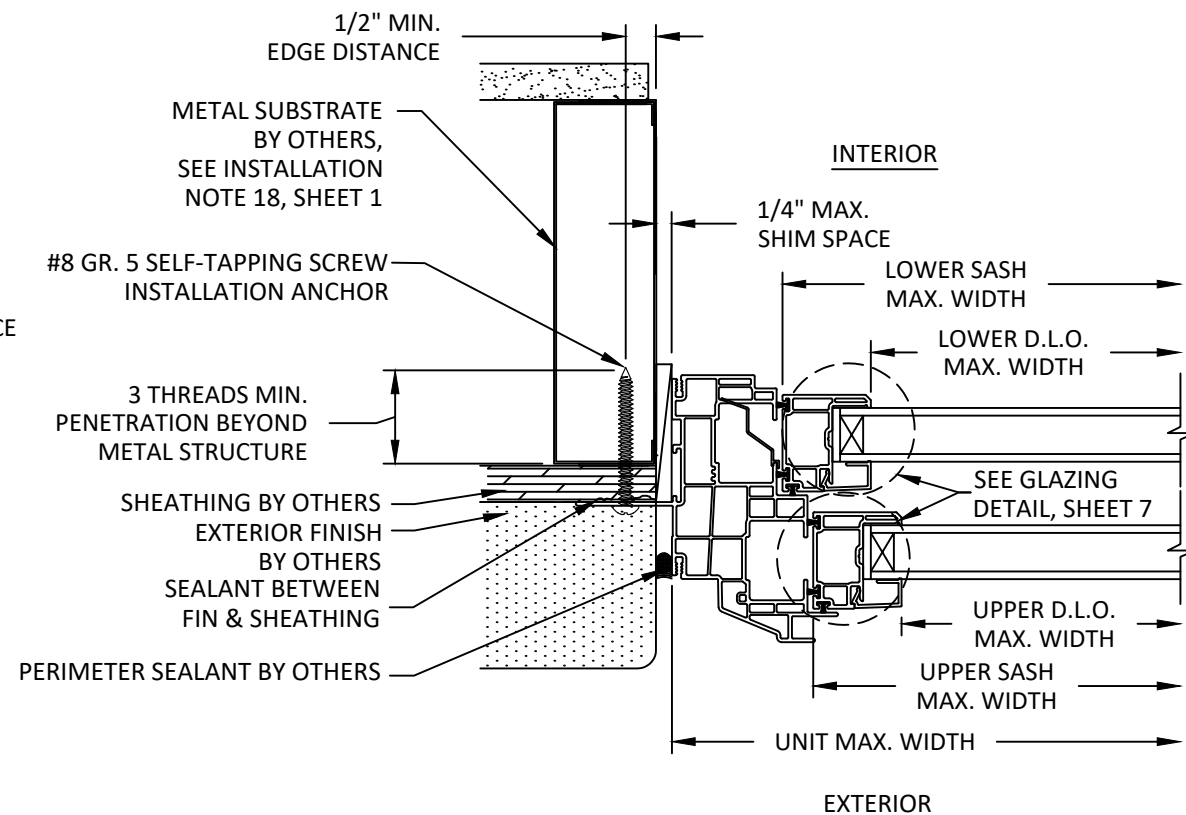
B 4 HORIZONTAL SECTION NAIL FIN INSTALLATION METAL STUD
