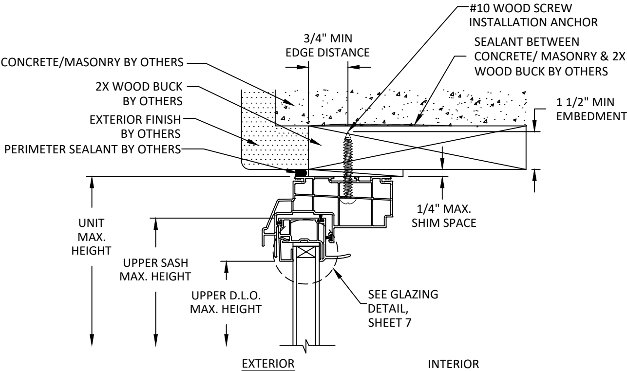
A 5 VERTICAL SECTION THROUGH FRAME INSTALLATION WOOD BUCK
