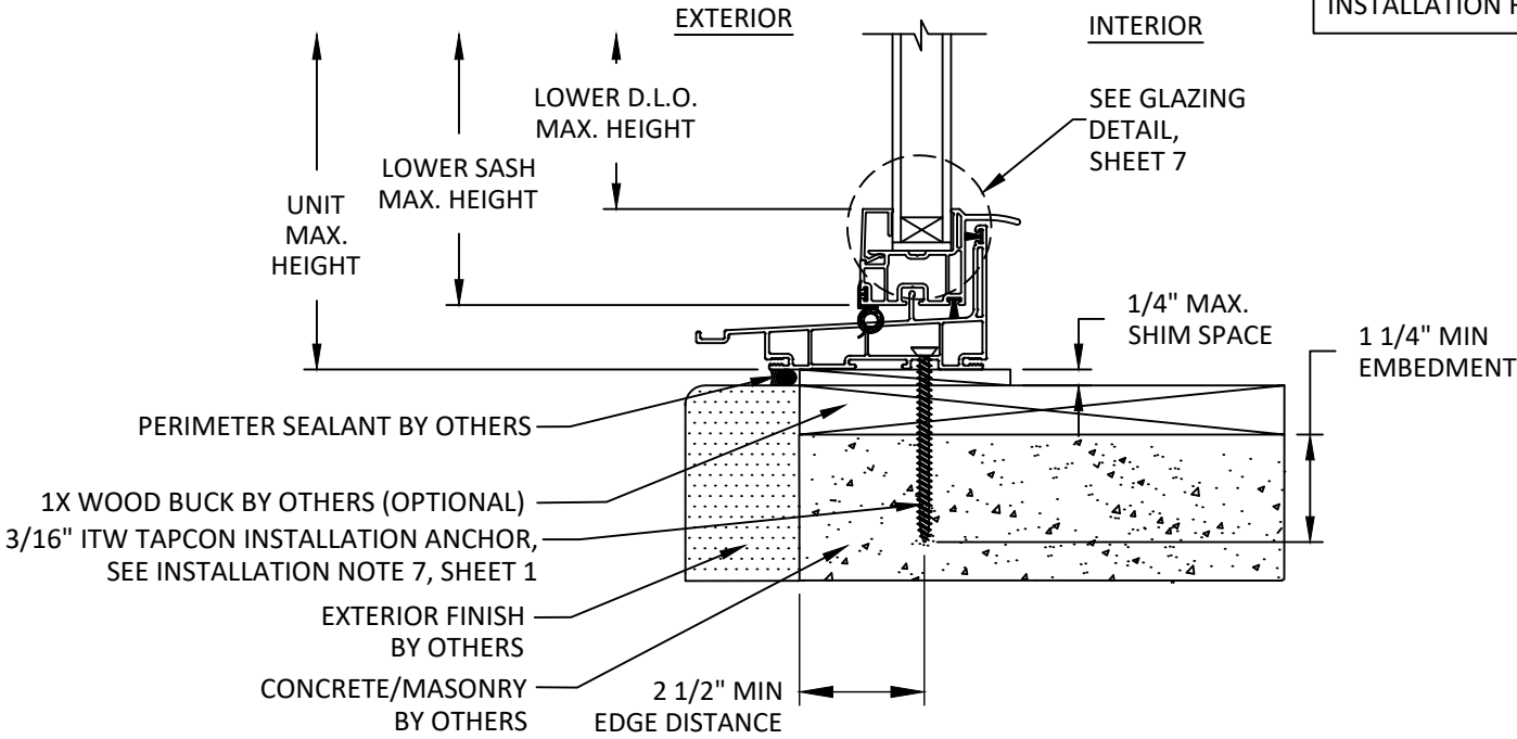
C 5 VERTICAL SECTION THROUGH FRAME INSTALLATION CONCRETE/CMU
