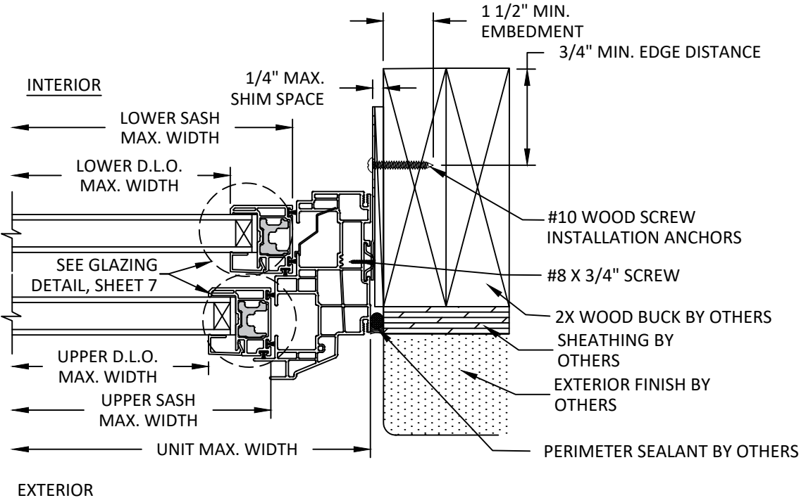
D 6 HORIZONTAL SECTION CLIP INSTALLATION WOOD BUCK
