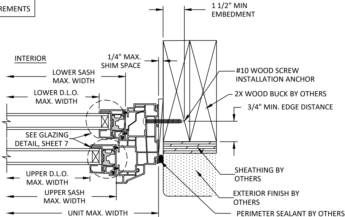
D 5 HORIZONTAL SECTION THROUGH FRAME INSTALLATION WOOD BUCK
