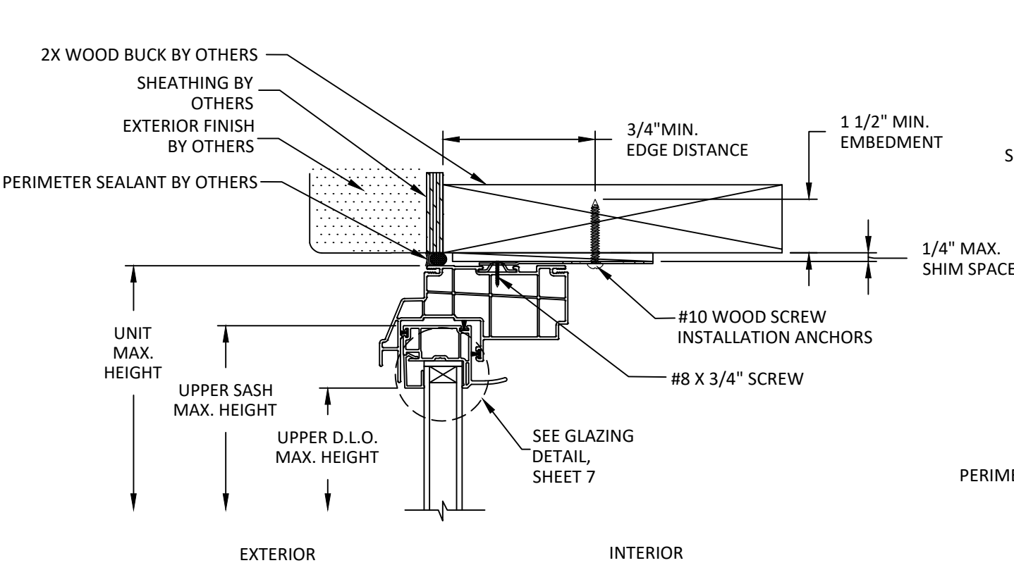
A 6 VERTICAL SECTION CLIP INSTALLATION WOOD BUCK
