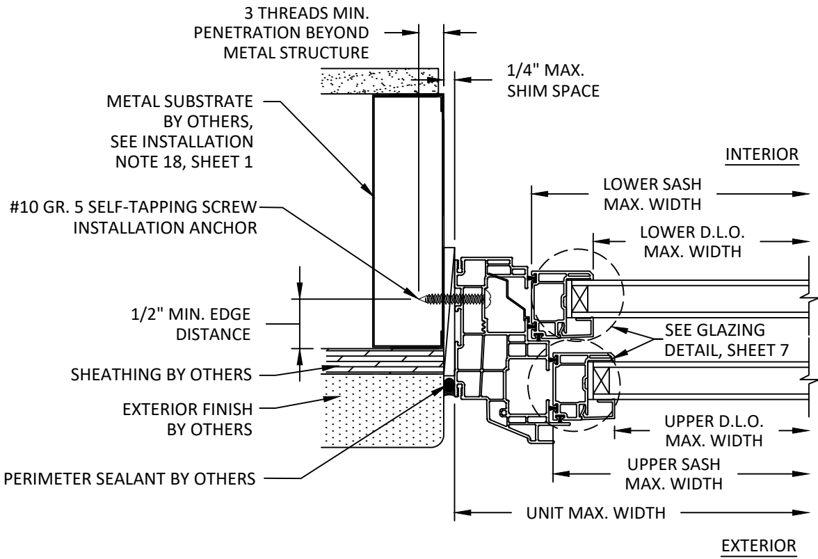
B 5 HORIZONTAL SECTION THROUGH FRAME INSTALLATION METAL STUD
